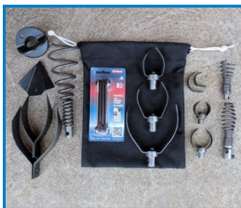
DRAWSTRING TOOL BAG MAIN LINE & SINK LINE TOOL KIT Item #129
